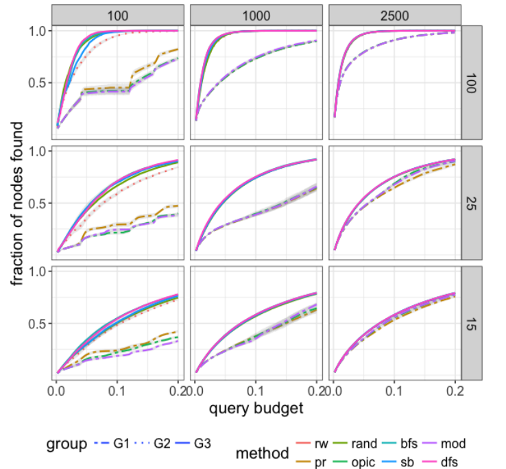
Figure 8: [Best viewed in color] Out Response : Results on networks with different values of average degree and community size ( \mu=0.1 ). G2 and G3 performance slightly increases when d_{avg} increases. G1 performance slightly improves as CS_{avg} increases, but it seems to be the worst performer in most cases.
