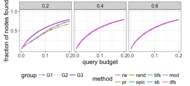
Figure 7: [Best viewed in color] Out Response : Results on networks with different \mu ( d=15 , CS=300 ). There is no difference in terms of performance for these methods on the networks with high community mixing.
