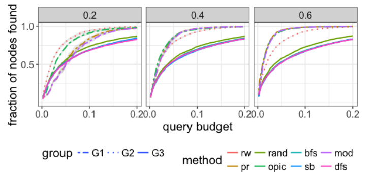
Figure 2: [Best viewed in color] Complete Resp.: Results on networks with different values of \mu ( d_{avg}=15 , CS_{avg}=300 ). G1 methods improve as \mu increases.
